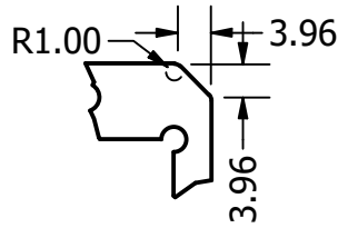
DETAIL D SCALE 1 : 1
